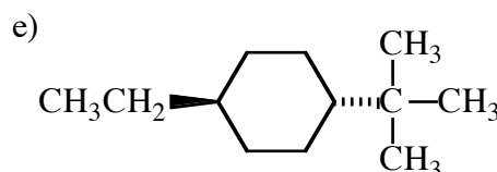
trans -1- tert -butyl-4-ethylcyclohexane
