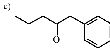
1-phenyl-2-pentanone
